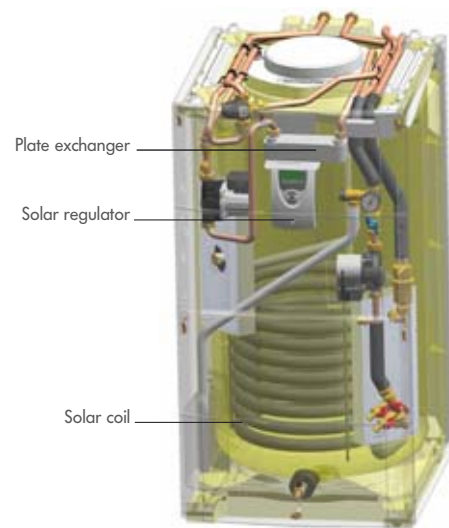
V 220 SHL DHW tank
